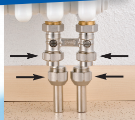
Cam for conically-sealing connection fittings
