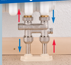
Flat-sealing straight-type diverter with shut-off capability for one- and two-pipe systems
