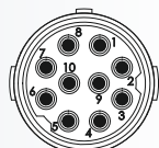
Insert pin mating view
